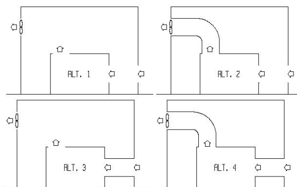
(1) VENTILATION PROPOSALS
